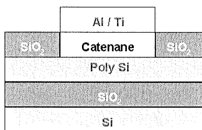
Fig. 2. 15 Molecular-based device
